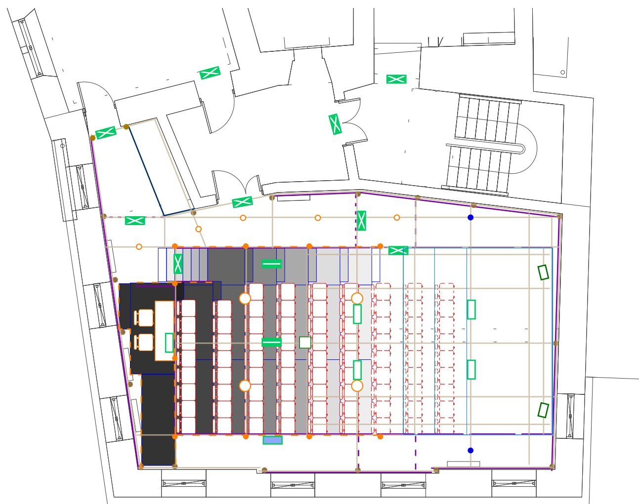
Additional units in crossover under control position and under seating deck
