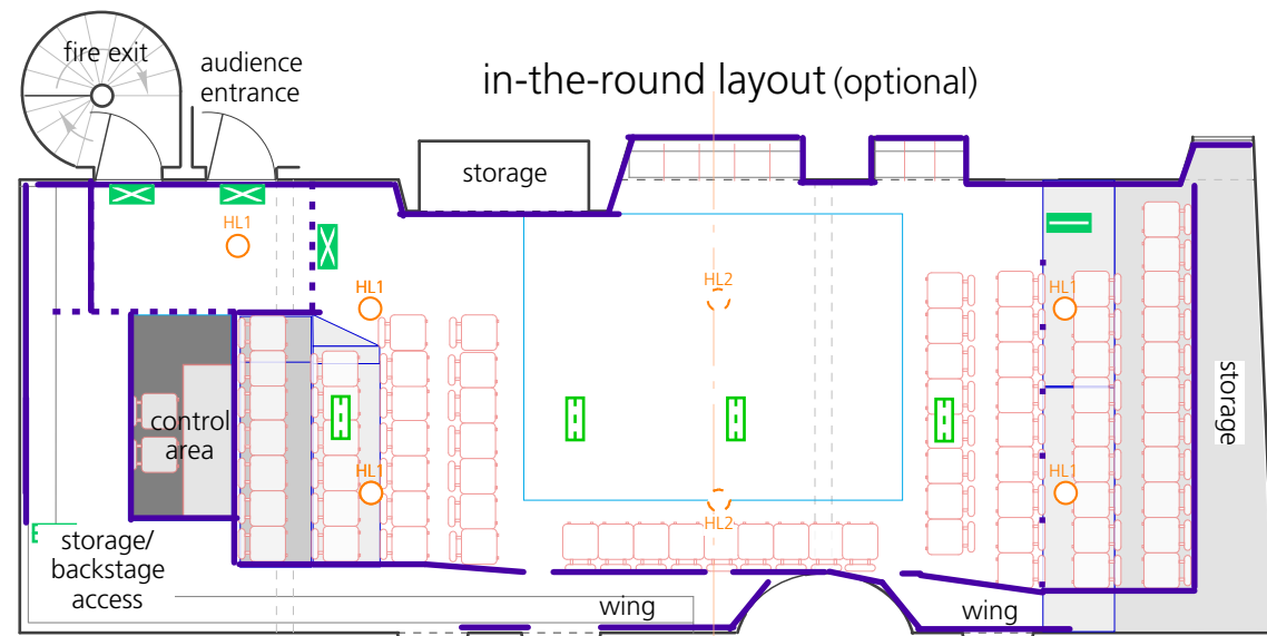
In-the-round layout (by arrangement) 79 seats approx
