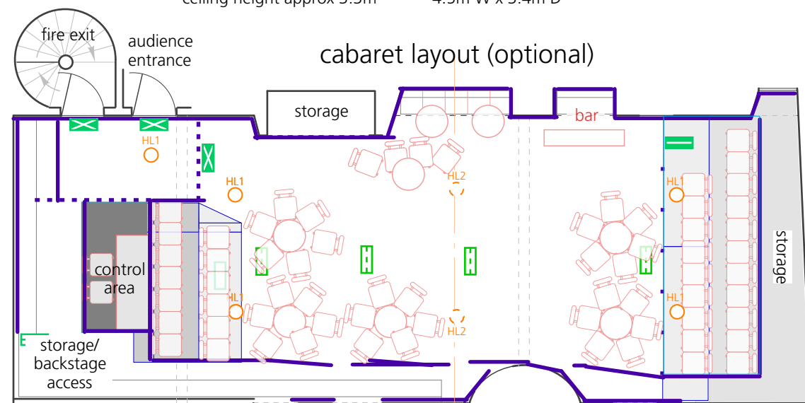
Cabaret layout (by arrangement) 72 seats approx Bar optional
